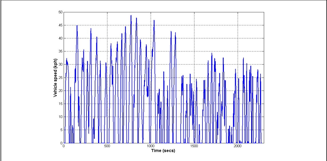
Fig. 11 | MTLB 159 Bus Cycle
