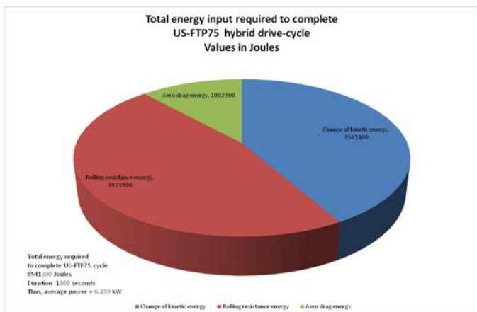
Figure 21 : Total Energy Required for the FTP75 in Joules
