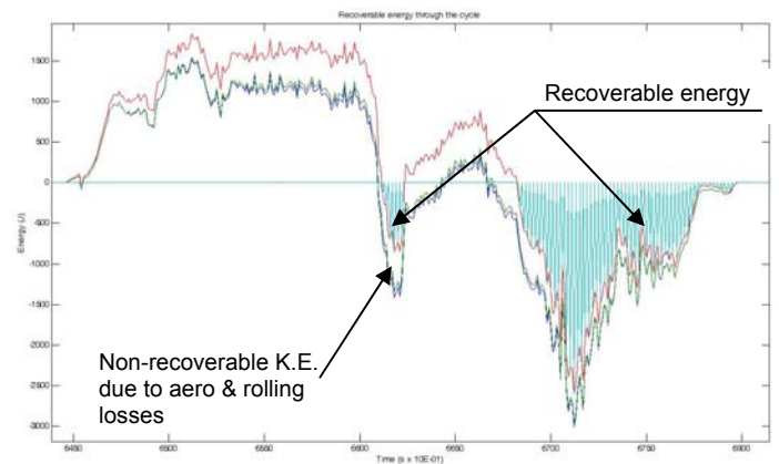
Figure 14 : Recoverable Energy - Expanded
