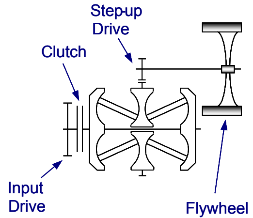
Figure 2: Schematic of Flywheel Hybrid System
