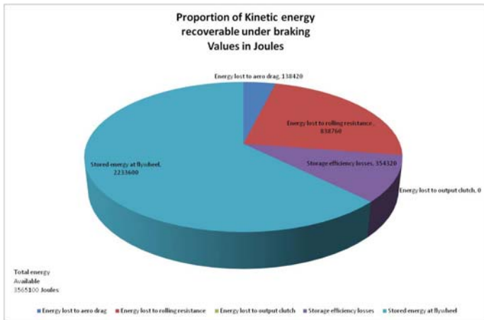
Figure 19 : Proportion of Energy Recovered in Joules
