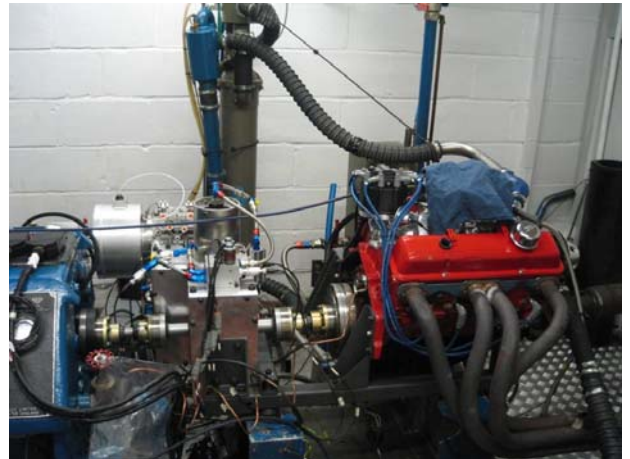
Figure 8: Dynamic Testing of the KERS
