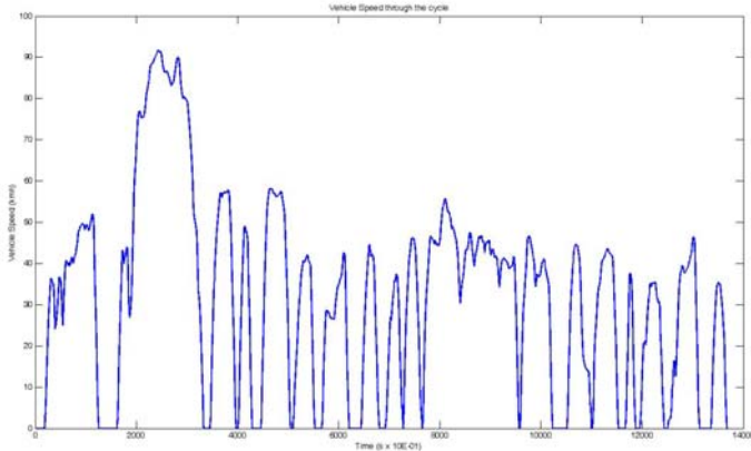
Figure 9: US-FTP75 cycle.
