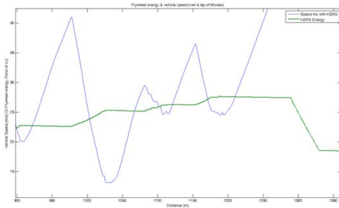
Figure 1: Vehicle Speed versus Flywheel Speed during a Formula One braking event during a lap of Monaco.
