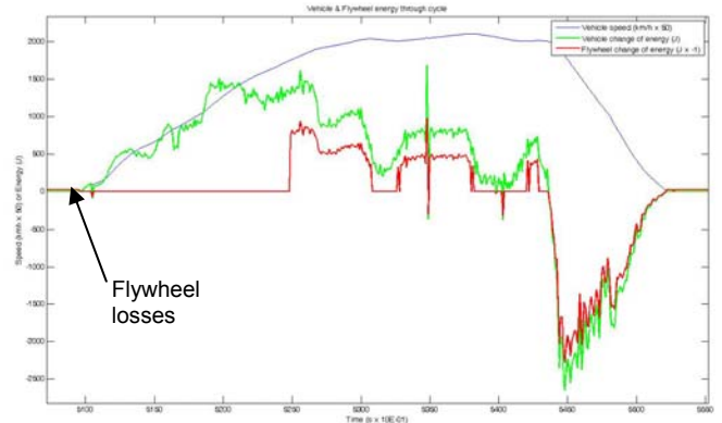
Figure 17 : Flywheel & Energy Changes – Expanded.
