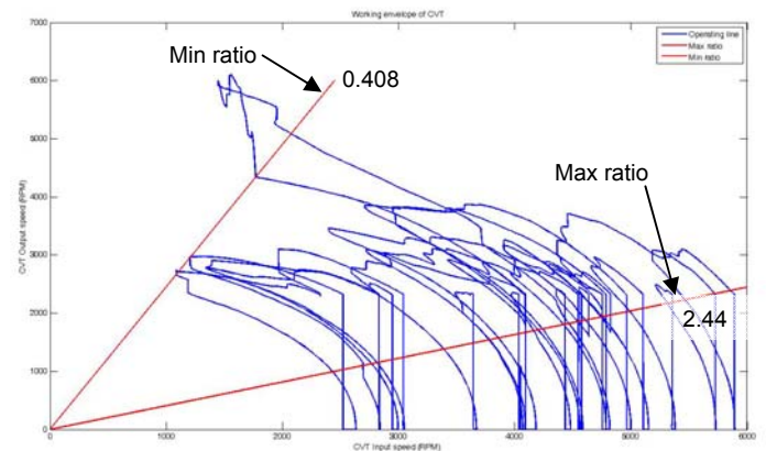
Figure 18 : CVT Ratio Envelope.
