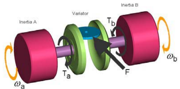
Figure 5: Principle of Torque Control
