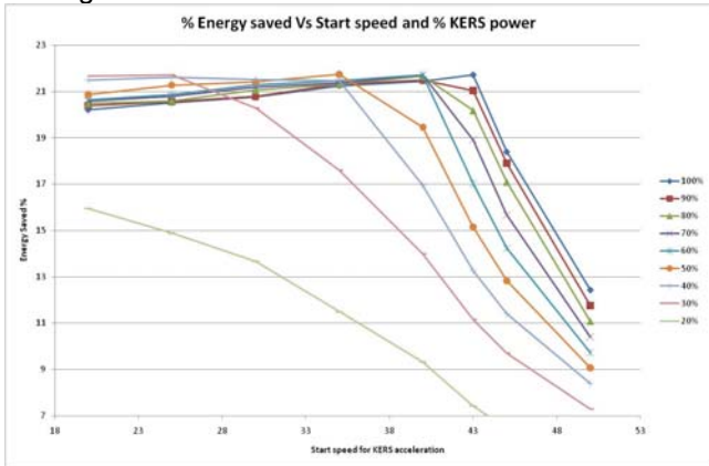
Figure 22: Variation of Energy Saved with Varying Strategy
