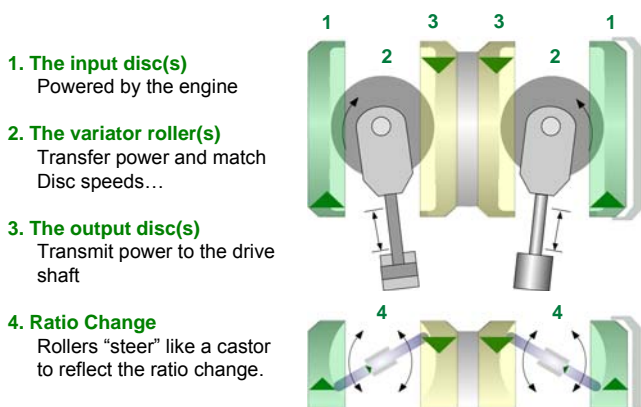
Figure 4: Full toroidal Variator schematic
