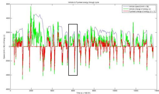
Figure 16 : Flywheel & Energy Change with Time
