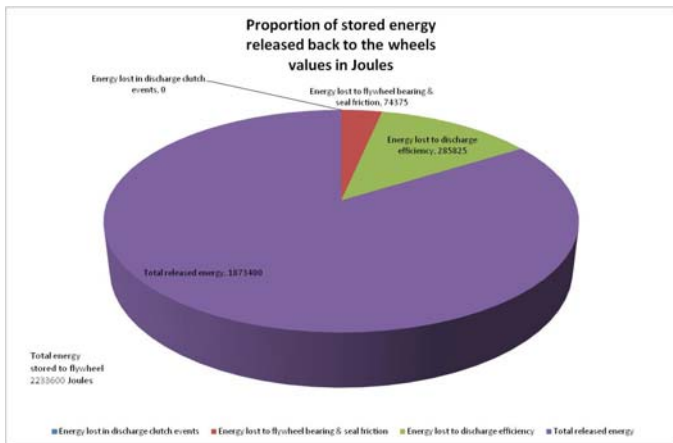
Figure 20 : Proportion of Energy Reapplied in Joules
