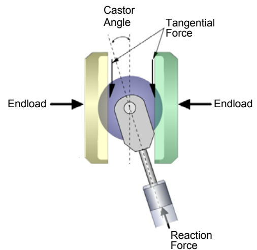
Figure 6: Variator Force Balance
