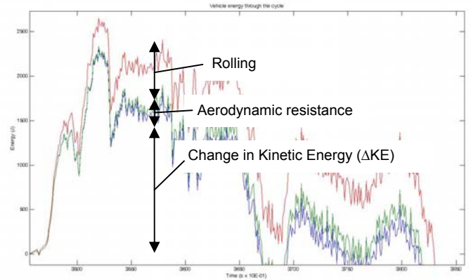
Figure 12: Energy Required to Propel the Vehicle
