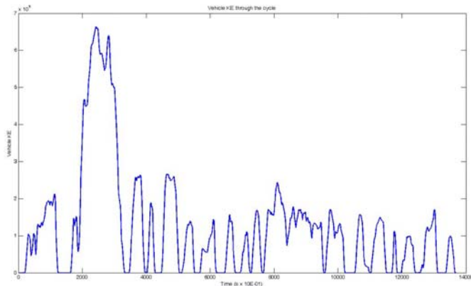
Figure 10: Vehicle Kinetic Energy over the FTP75 cycle.
